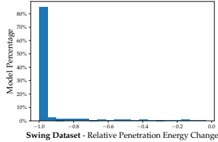
Figure 5: The histogram of relative penetration energy change for successful examples in the Swing dataset. Our method achieves a success rate of 85.1%, and we observed an average relative decrease of 94.3% in penetration energy.
